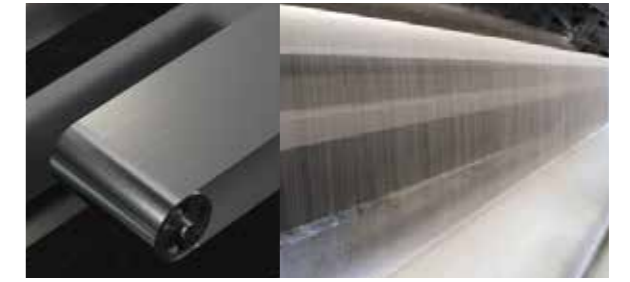
薄膜流延 Film Casting
